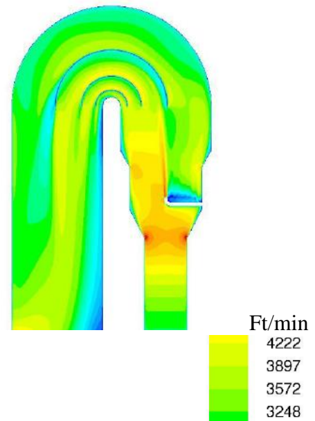
Venturi CFD Model
