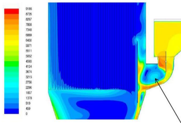
Typical CFD compartment flow model
